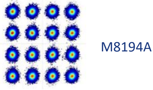
96 GBd 16QAM – 768 GBit/s EVM 6.8%
