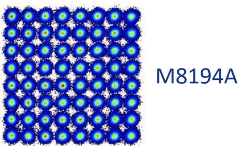
80 GBd 64QAM - 960 GBit/s EVM 4.4%
