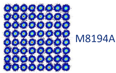
64 GBd 64QAM - 768 GBit/s EVM 3.8%
