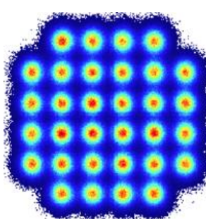
160 GBd 32QAM – 1.6 TBit/s EVM 11.5%
