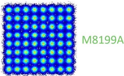
110 GBd 64QAM – 1.32 TBit/s EVM 6.3%
